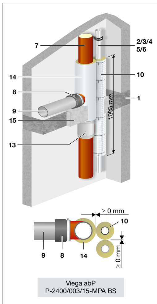
Fig. 42: Example – Saint Gobain HES SVB plug connector installation acc. to Z-19.17-2130, system 4, pipe run \leq 160 mm
