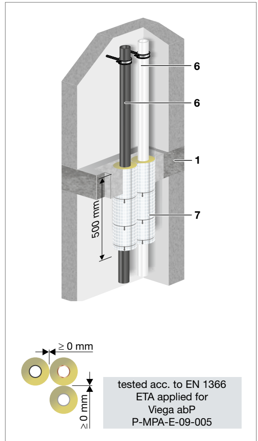
Fig. 32: Zero clearance Viega piping systems
