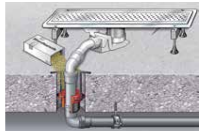
Fig. 106: Pipe lead-in with Advantix shower channel
