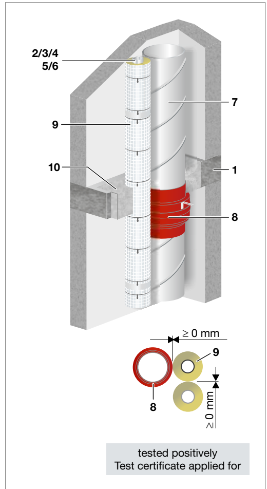
Fig. 56: Shut-off devices K 90-18017-3 – Wildeboer TS 18
