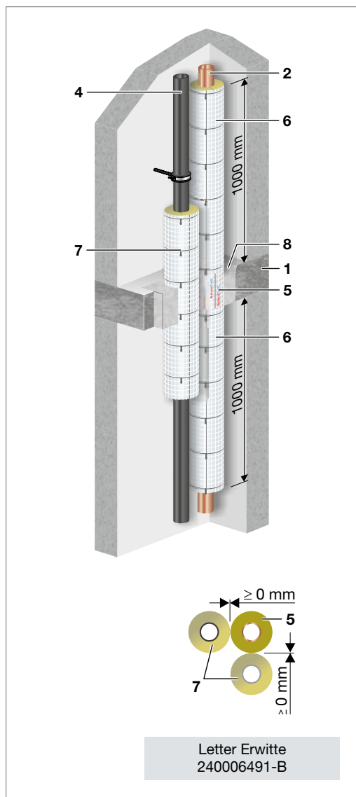
Fig. 37: Viega plastic piping system to non-combustible pipes with Rockwool Conlit 150 U, abP P-3725/4130_MPA BS
