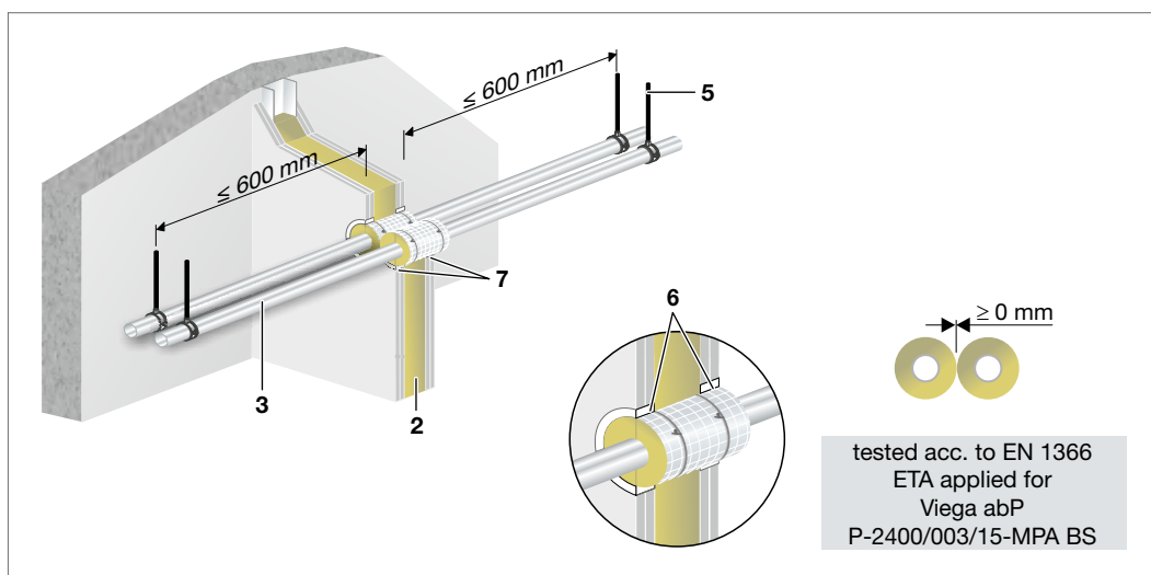
Fig. 65: Raxinox – Installation in light-weight partition
