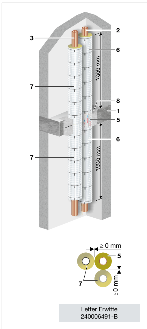
Fig. 36: Viega metal piping system to non-combustible pipes with Rockwool Conlit 150 U, abP P-3725/4130_MPA BS
