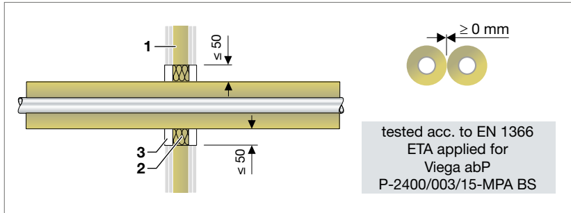
Fig. 75: Filling with loose rock wool/gypsum filler
