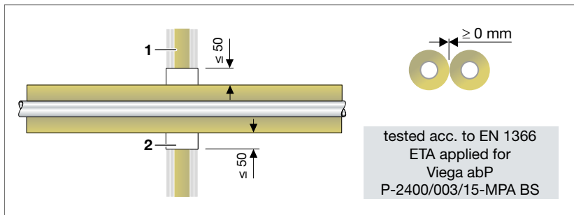
Fig. 76: Filling with gypsum filler
