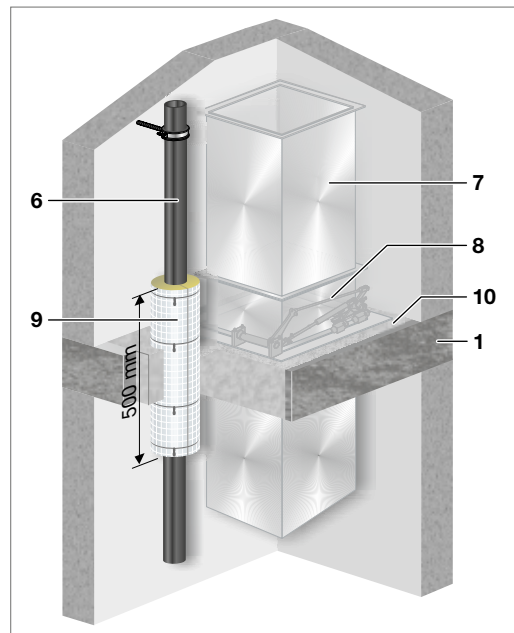
Fig. 58: Fire dampers/EN1366-2
