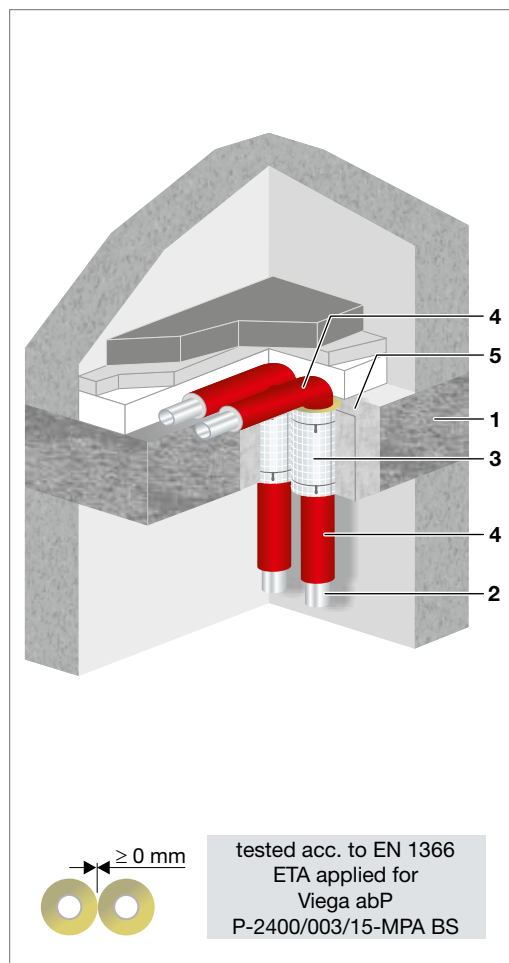
Fig. 28: Offset in the floor construction
