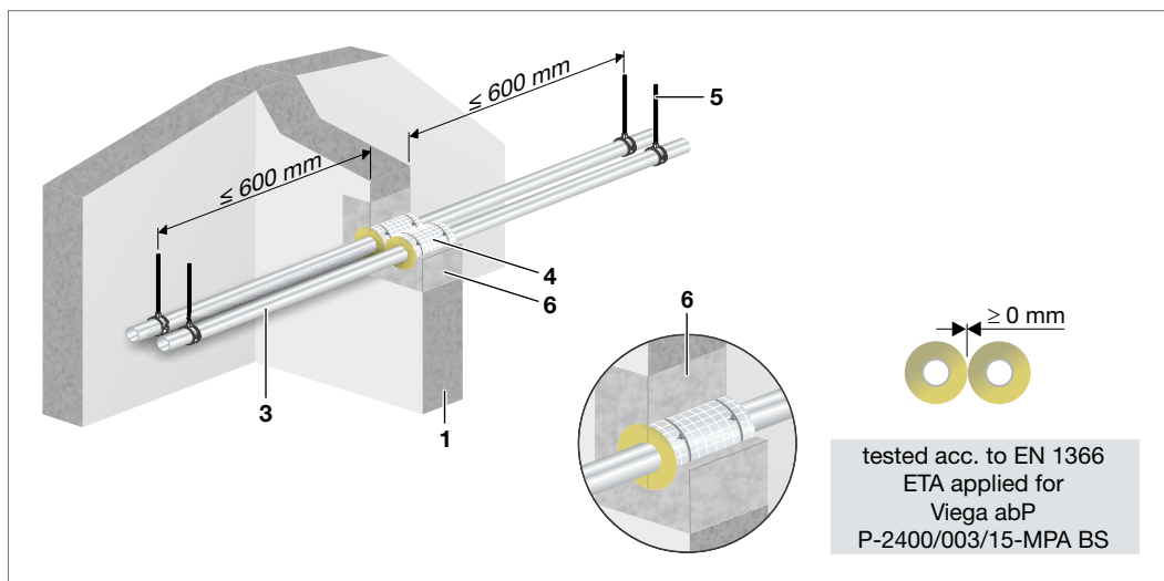
Fig. 64: Raxinox – Installation in solid wall
