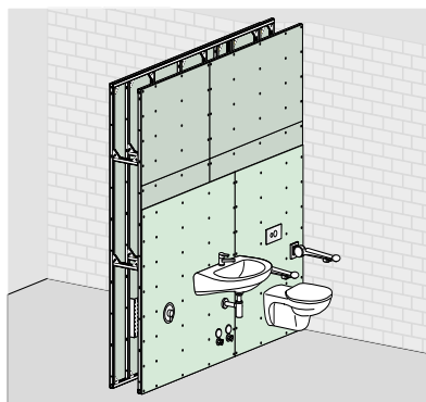
Fig. 96: Steptec partition with cladding
