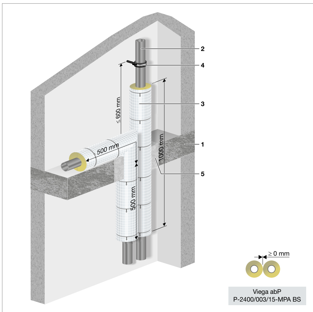
Abb. 96: Megapress
