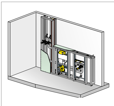
Abb. 292: Viega Prevista Dry – Vorwandmontage
